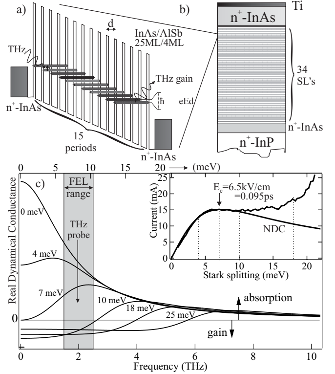
FIG. 1: (a) The superlattice structure under dc bias sandwiched between two n^+ regions. (b) Super-superlattice mesa structure is a repetition of 34 cells depicted in (a). (c) Real dynamical conductance, dI/dV , versus frequency for different applied electric fields using scattering parameters consistent with the DC I-V shown in the inset. Electric fields are given in units of the energy spacing of the Stark ladder states.
