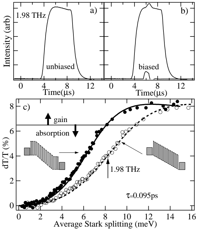
FIG. 3: (a) A pulse of terahertz radiation is transmitted and detected. (b) A short electrical pulse applied to the super-superlattices causes an increase in transmission. (c) Solid circles display the fractional change in transmission as a function of applied voltage displayed as the average voltage drop per quantum well. The predicted dependence based on Fig. 1(c), is shown by the dashed curve. The experimental data can be brought into agreement (open circles) if .75 of the quantum wells experience a Stark splitting. The schematic superlattice to the right is uniformly biased; to the left the same voltage drop appears over fraction of the quantum wells between two n+ regions. The model indicates that the cross over from loss to gain occurs at different values of the fractional change in transmission.
