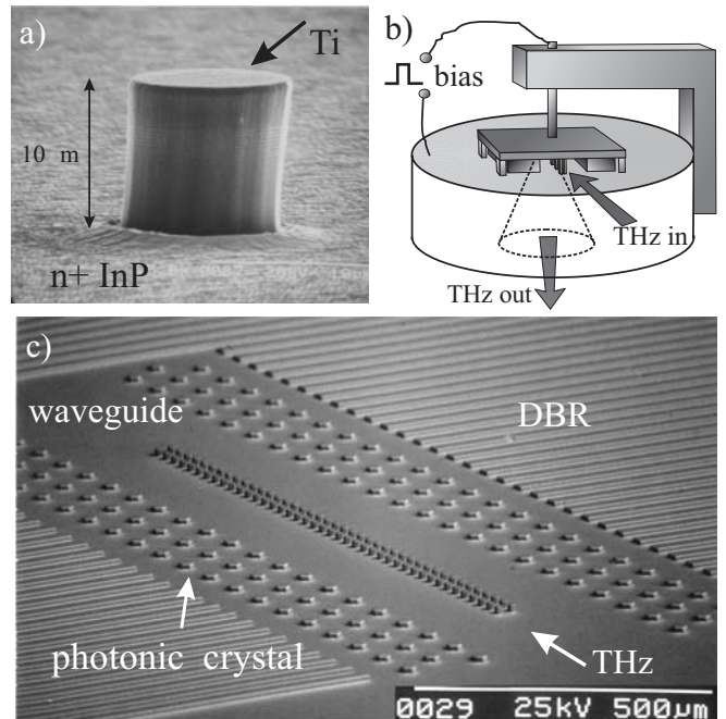
FIG. 2: (a) Super-superlattice mesa. (b) A schematic of the structure in (c) pressed onto the metal surface with a hole to form a waveguide and out-coupling hole. (c) Waveguide without the top metal. A double row of super-superlattice mesas in the middle of the waveguide. Sidewalls are defined by a photonic bandgap structure.
